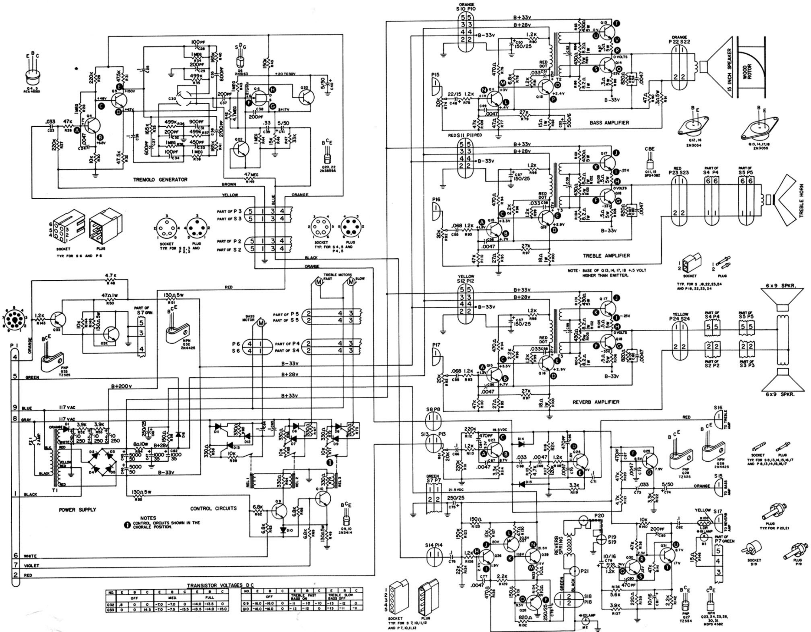
Figure 28. Schematic, LESLIE Speaker Model 910
