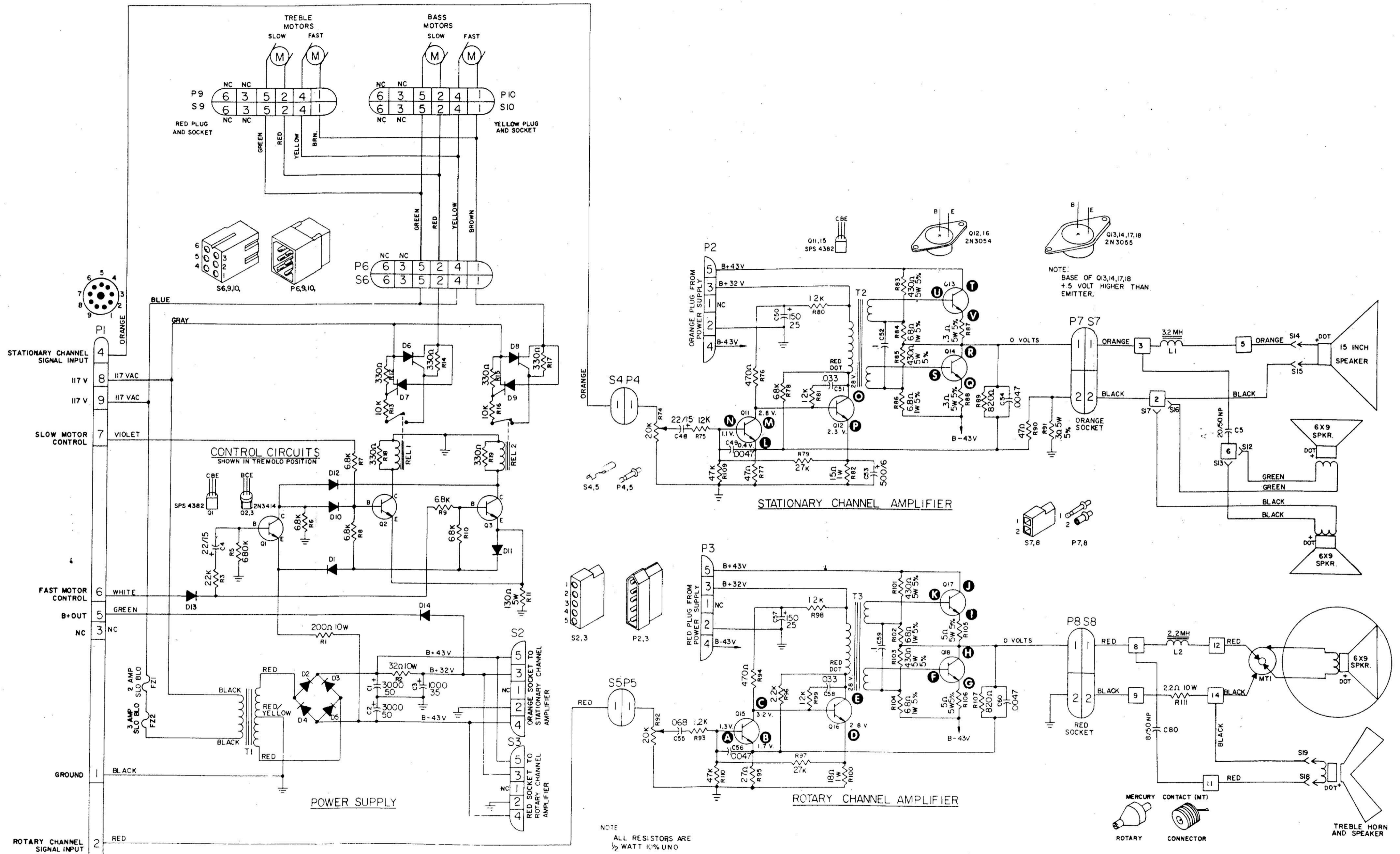
Figure 34. LESLIE Speaker Model 710 Schematic
